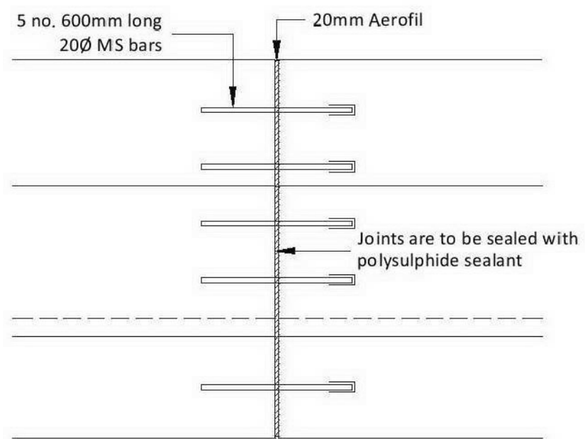
EXPANSION JOINT DETAIL Scale 1:20 Joints at 6m crs. Expansion joints at 24m crs
